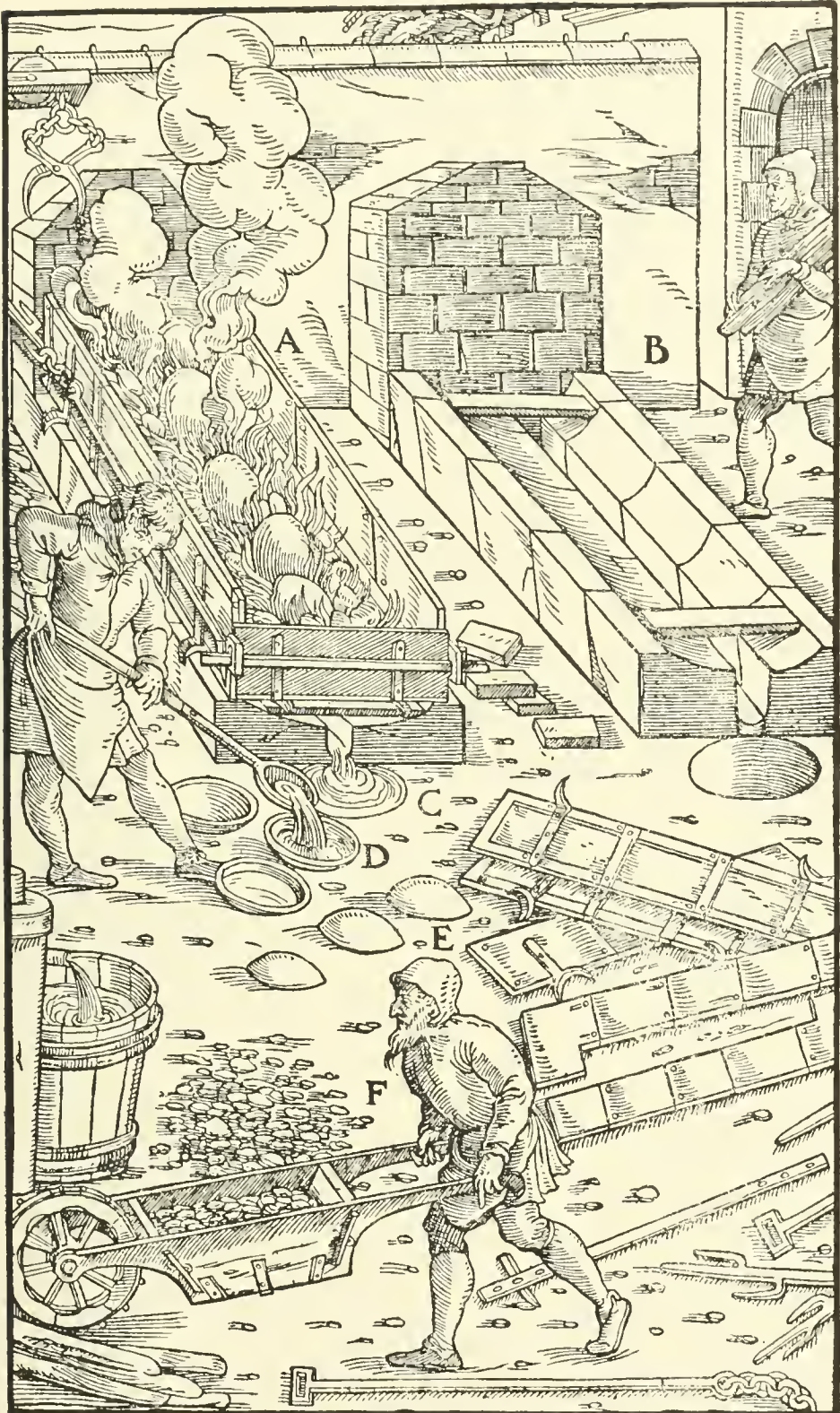
A — FURNACE IN WHICH THE OPERATION OF LIQUATION IS BEING PERFORMED. B — FURNACE IN WHICH IT IS NOT BEING PERFORMED. C — RECEIVING-PIT. D — MOULDS. E — CAKES. F — LIQUATION THORNS.
